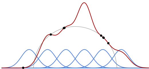
Figure 1.2: If the amount of training data (black dots) is small compared to the capacity of the model, the empirical performance of the fitted model (red curve) during training reflects poorly its actual fit to the underlying data structure (thin black curve), and consequently its usefulness for prediction.
